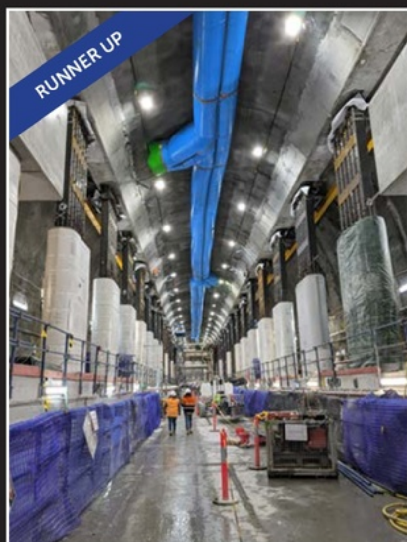
Construction of cavern lining works in the Town Hall Station cavern beneath Swanston Street. Melbourne Metro Tunnel Project, by Vern Lee
